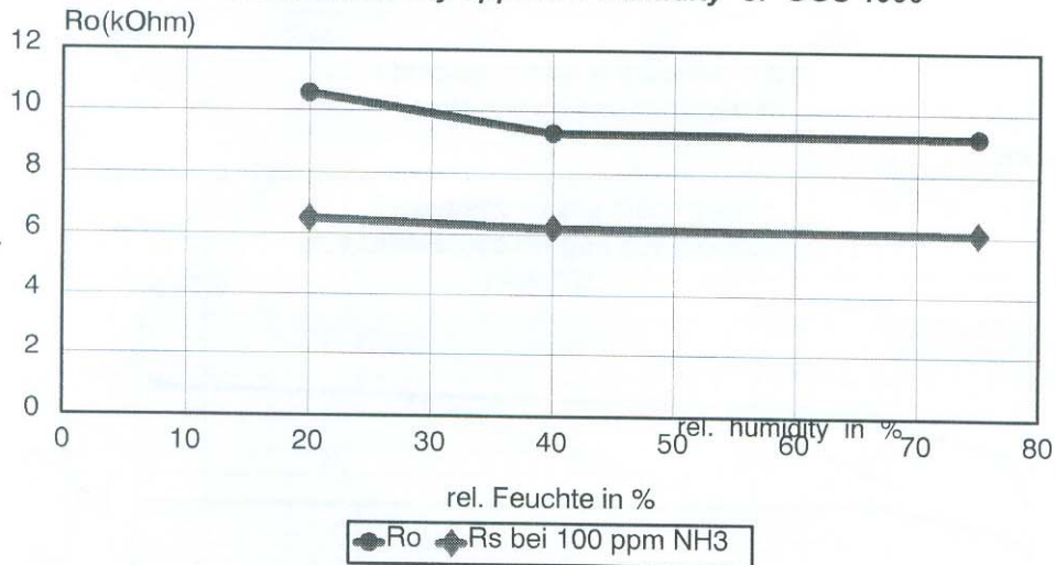
cross sensitivity opposite humidity of GGS 4000
