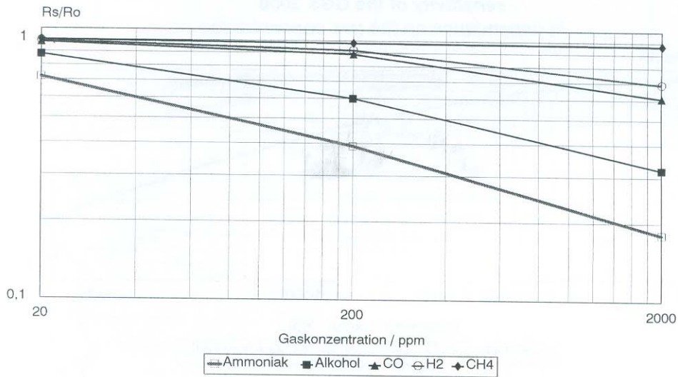
sensitivity of GGS 4000 in dependence on the gas concentration
