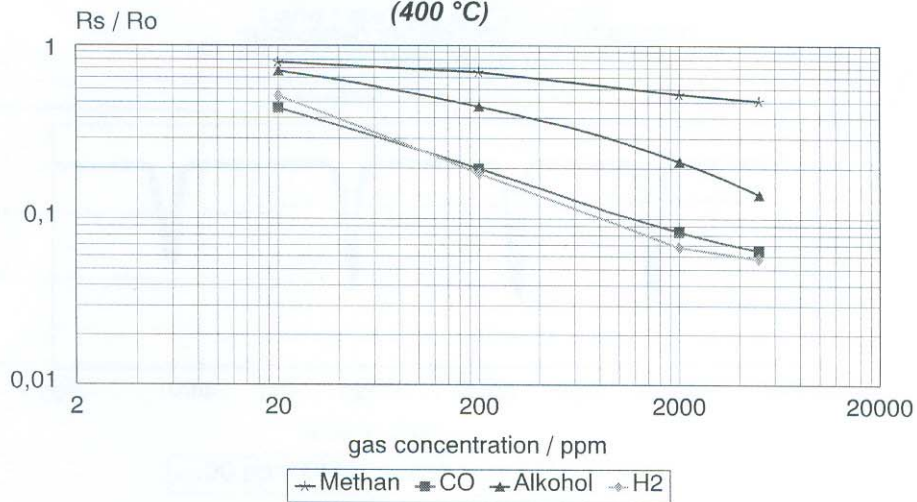
Sensitivity of the GGS 2000 in dependence on gas concentration (400 ^{\circ}\text{C} )
