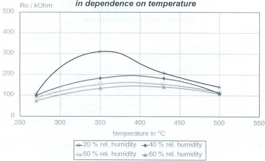
Sensitivity of the GGS 2000 in dependence on temperature
