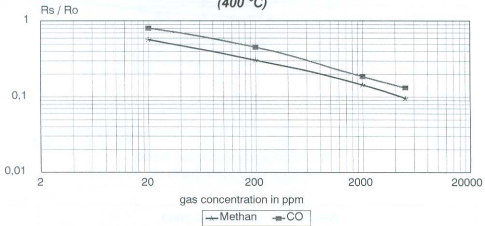
Sensitivity of GGS 1000 in dependence on gas concentration (400 °C)
