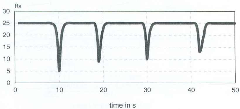
response time and decay behaviour of GGS 1000
