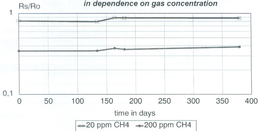
Long time test of GGS 1000 in dependence on gas concentration
