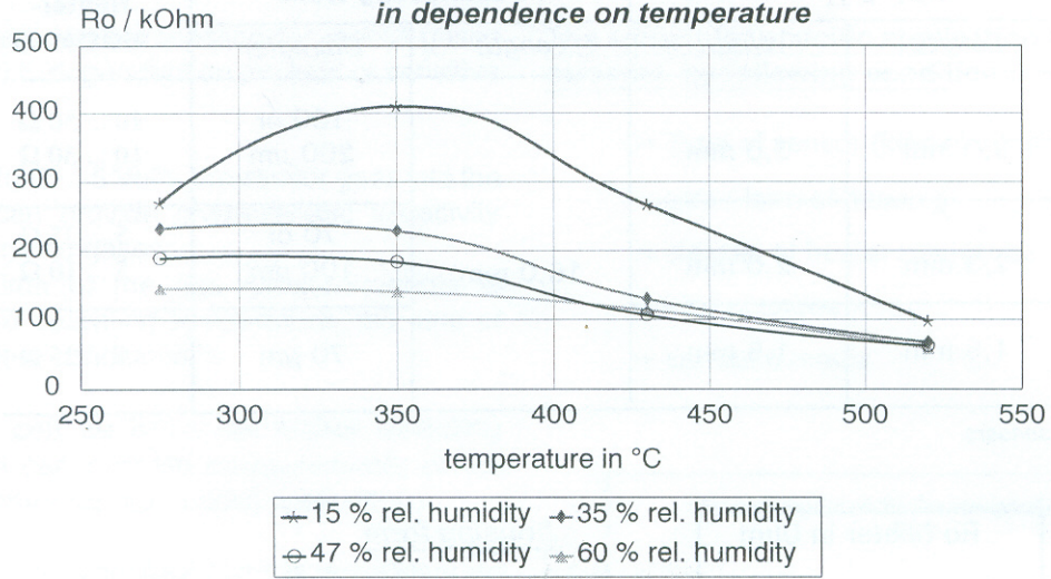
Sensitivity of the GGS 1000 in dependence on temperature
