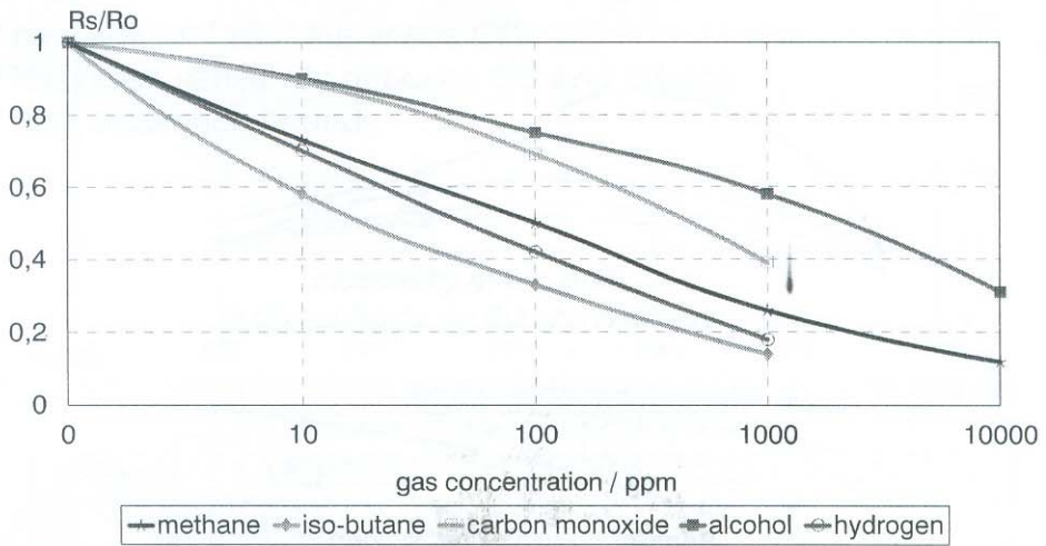
Sensitivity of GGS 1000 opposite various kinds of gas
